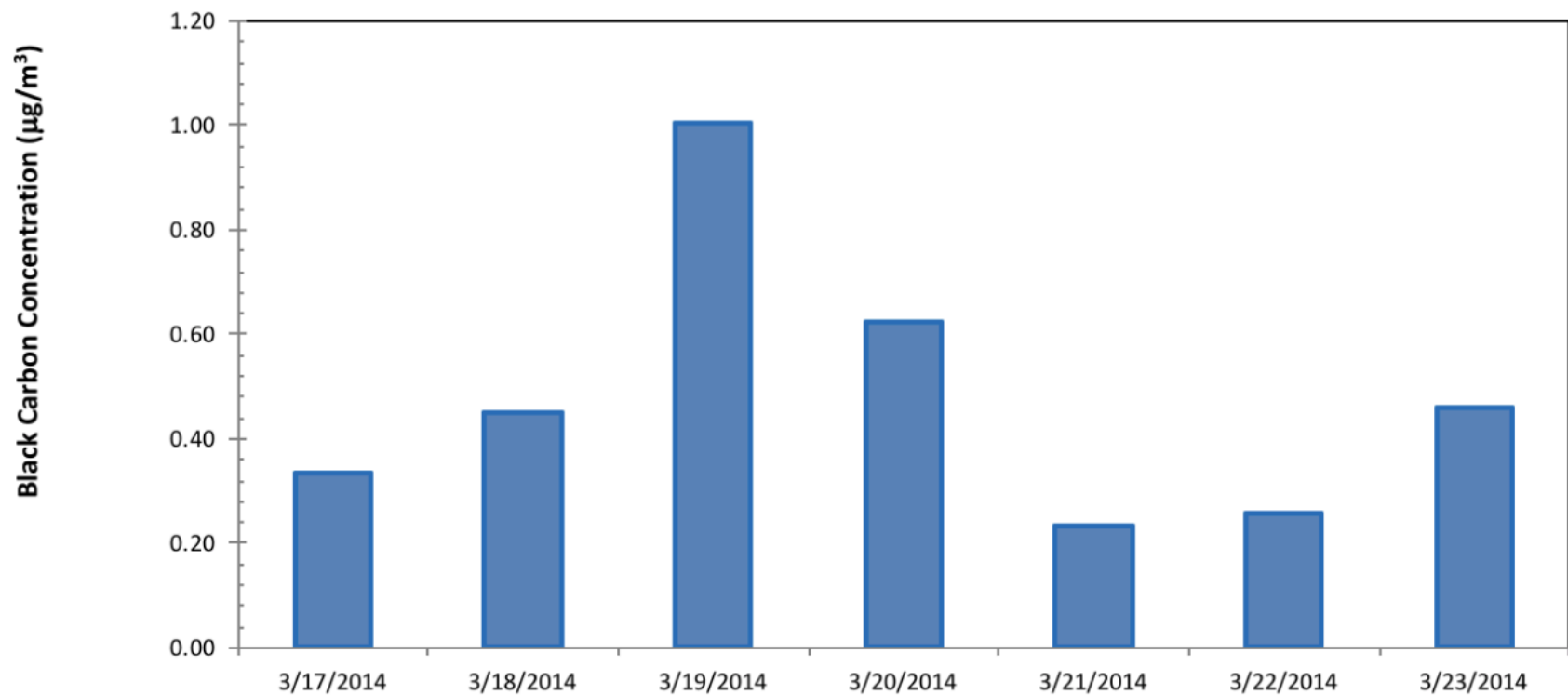
Figure 4. Daily black carbon concentration averages in National City for seven days as sampled by MicroAeth .
